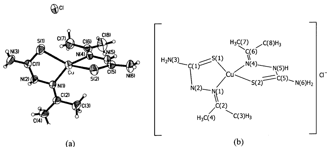
Figure 1. (a) Perspective view of complex 1 with thermal ellipsoids at the 50% probability level; (b) structural formula
