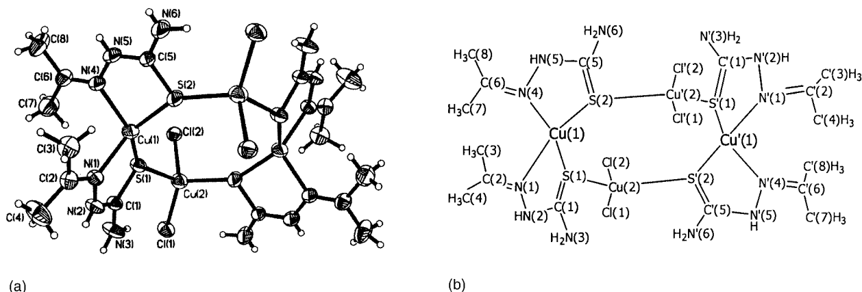
Figure 2. (a) Perspective view of complex 2 with thermal ellipsoids at the 50% probability level; (b) structural formula
