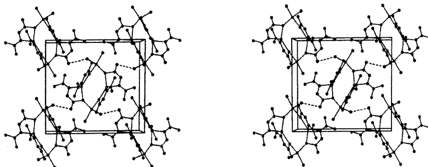
Figure 3. A stereoscopic view of the packing in the unit cell of [\text{Cu}_2\text{Cl}_2(\text{tscac})_2]_2 ( 2 ) showing the intermolecular hydrogen bonding
